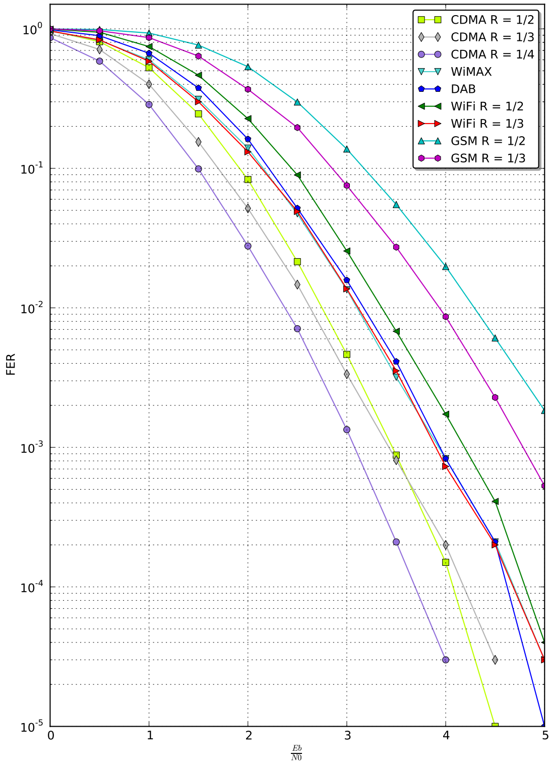
Figure 4.9: Standards overview; Frame length = 400; Input bit length = 4; No windowing
