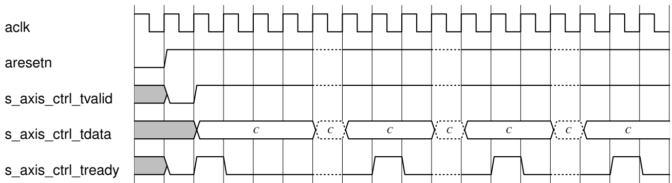
Figure 2.3: Fixed decoder configuration
