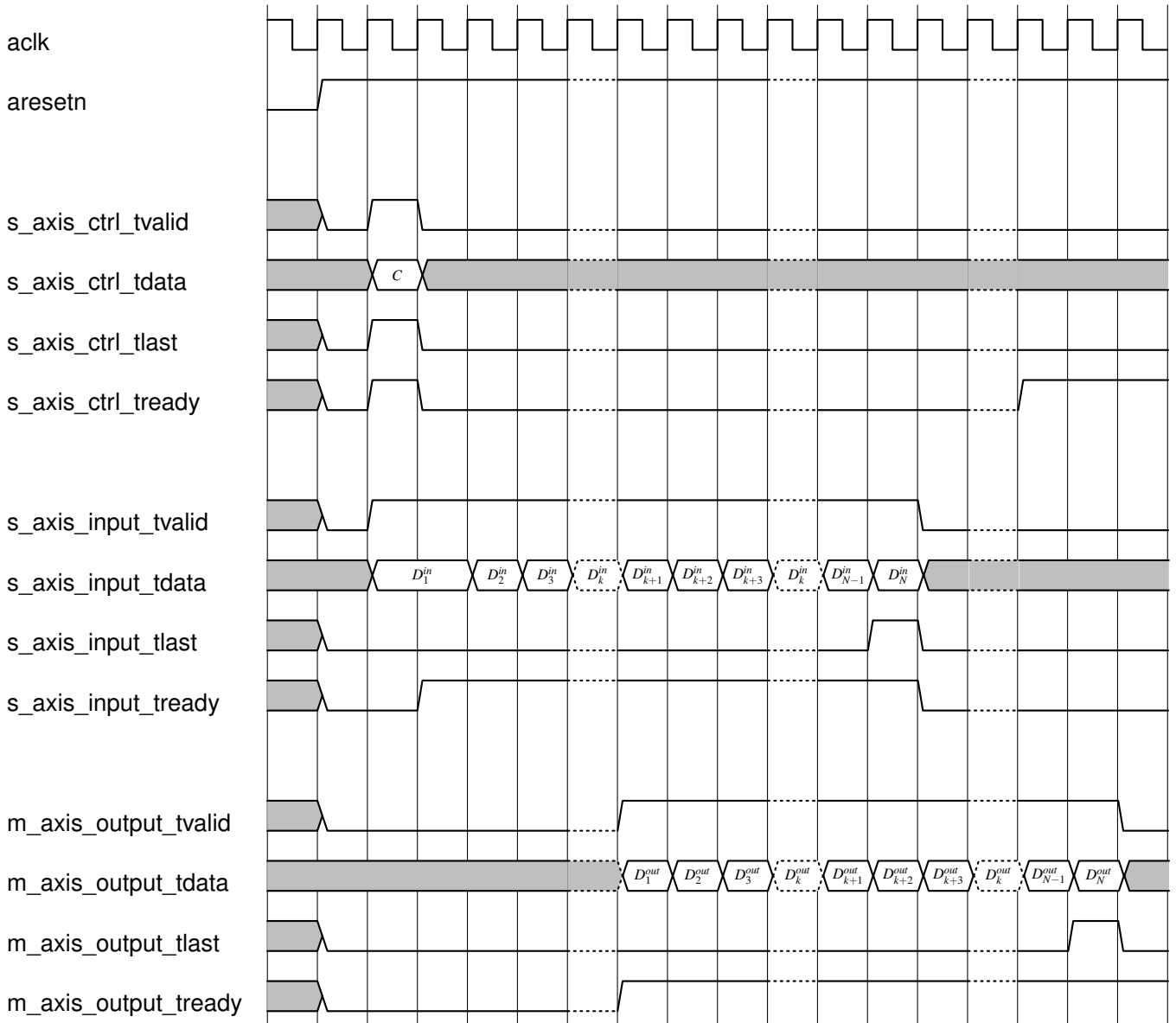
Figure 2.2: Decoder timing for configuration, data input and output
