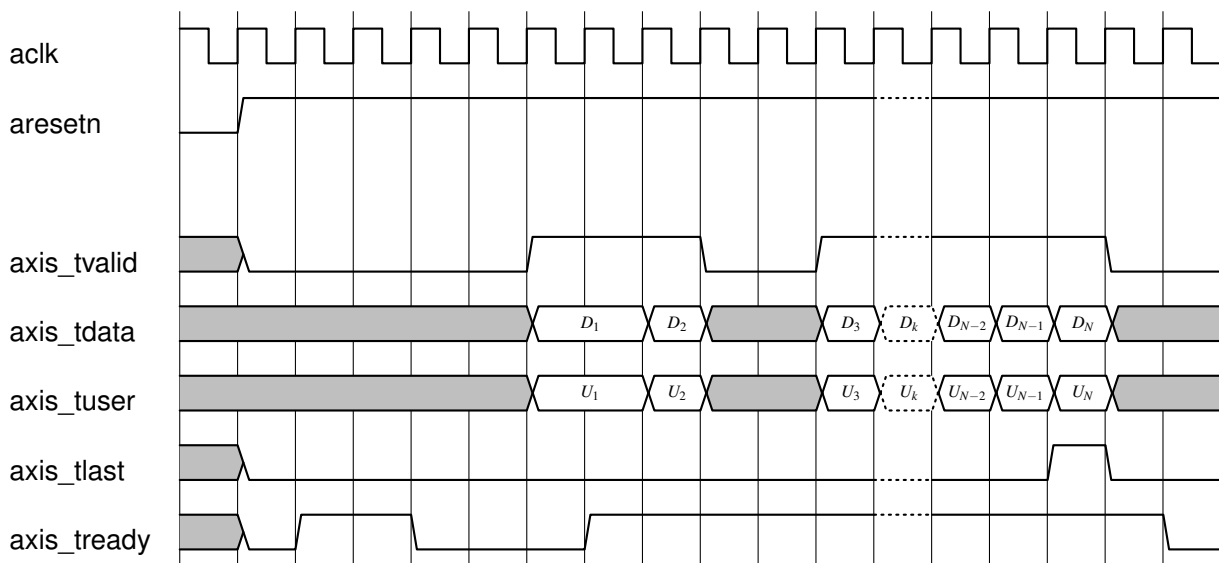
Figure 2.1: Example of an AXI4-Stream handshake
