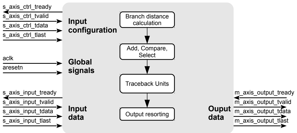
Figure 1.1: Block diagram of the Viterbi decoder
